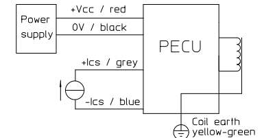
Connection diagram for 4-20mA control signal fig.2b
