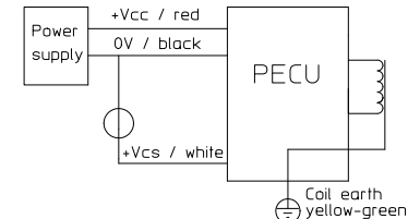
Connection diagram for 0-10V control signal fig.2a
